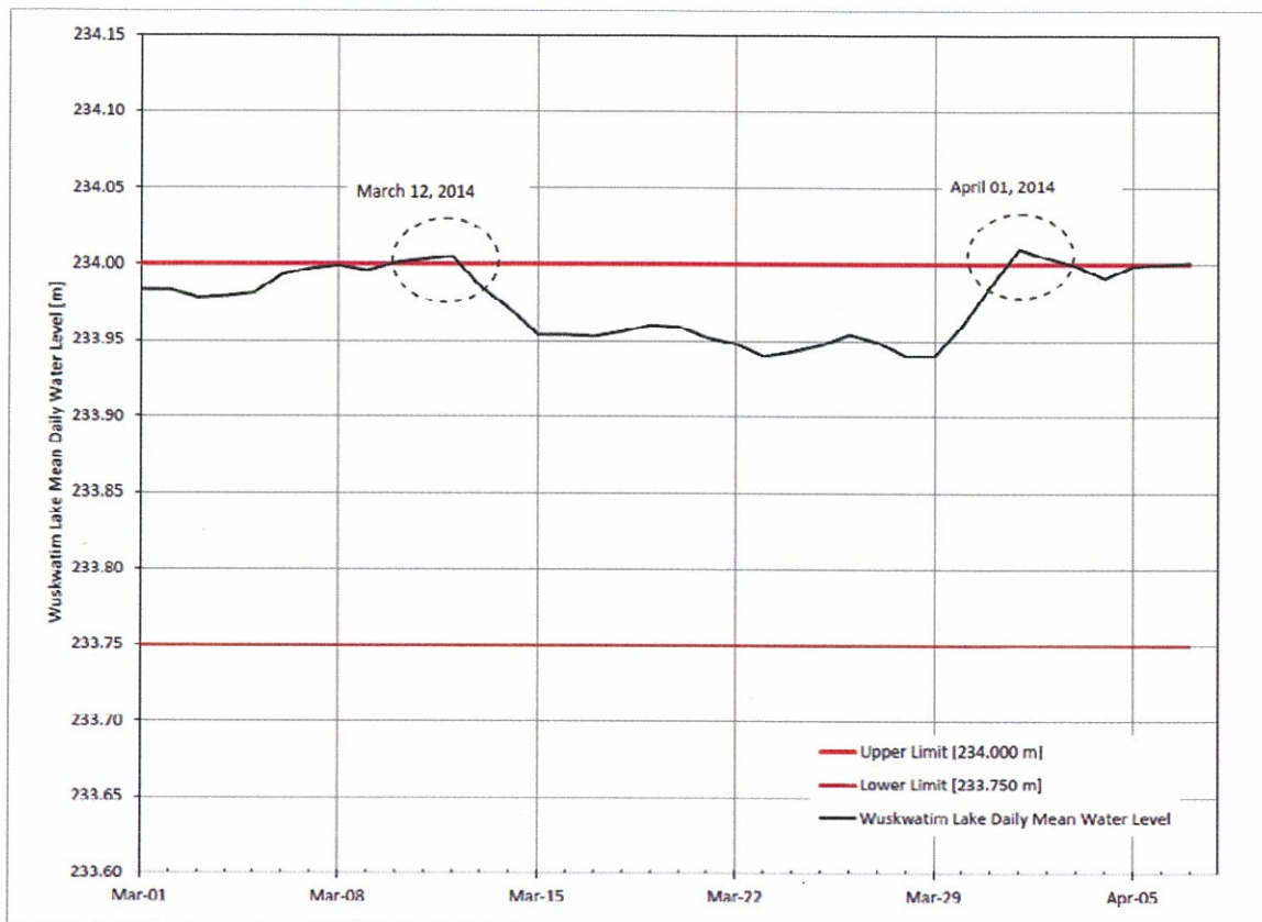
Figure 1: Wuskwatim Lake Mean Daily Water Level (with wind and wave effects eliminated)
