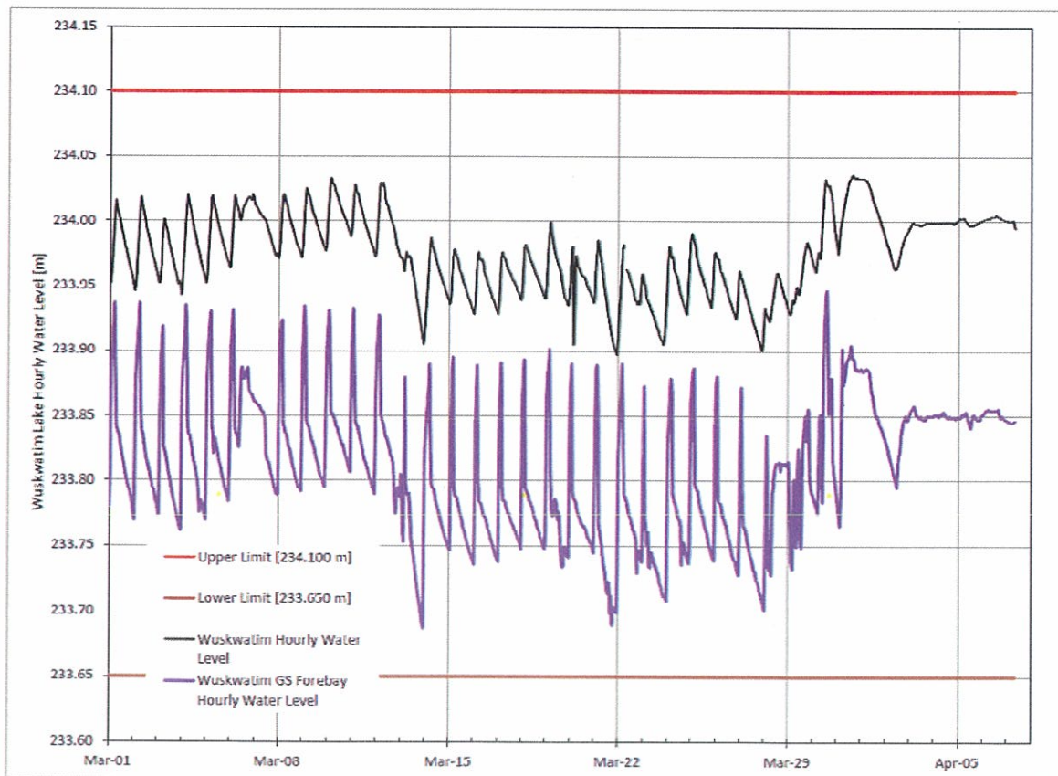
Figure 2: Wuskwatim Hourly Water Levels and Generating Station Forebay Hourly Water Level
